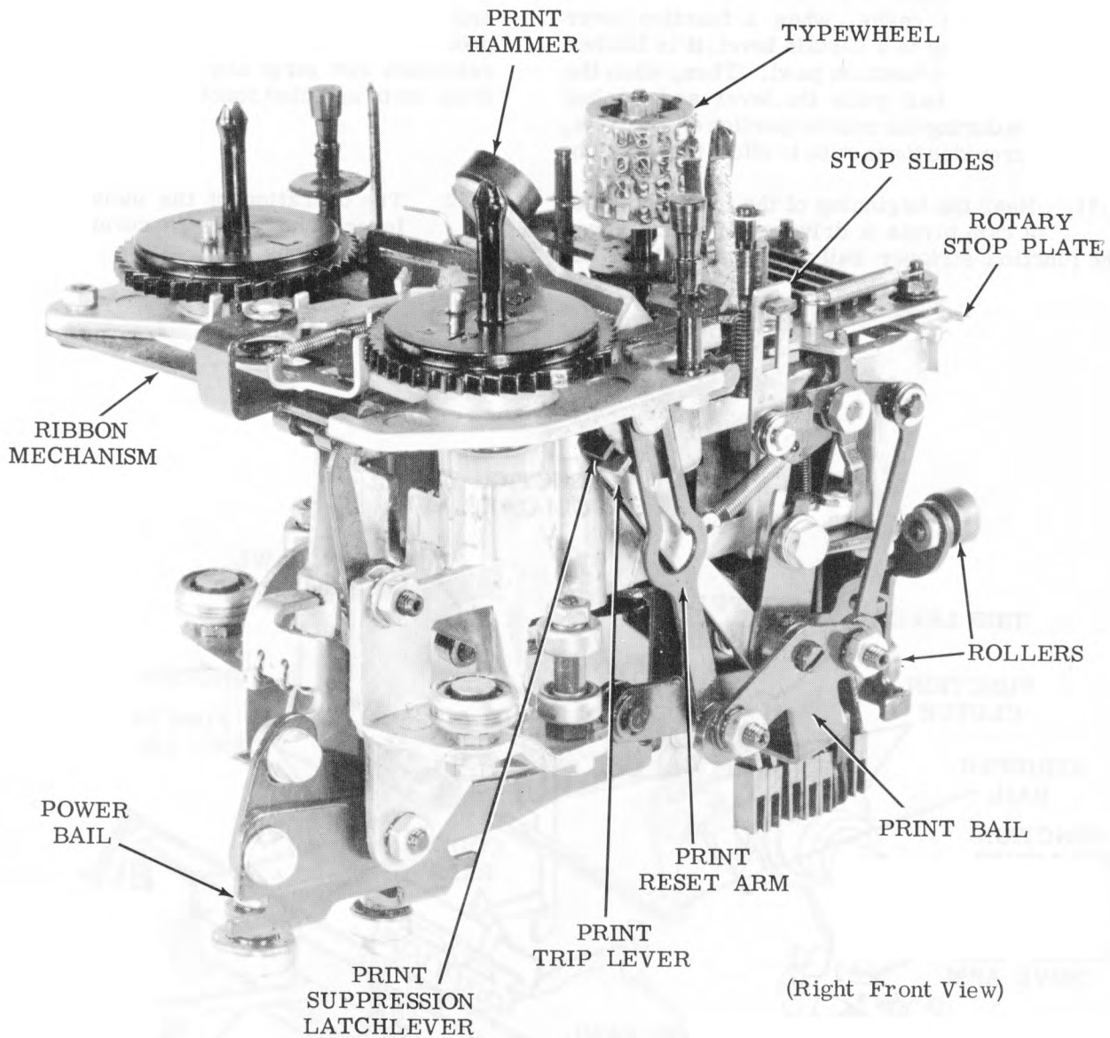
Figure 18 - Print Carriage
