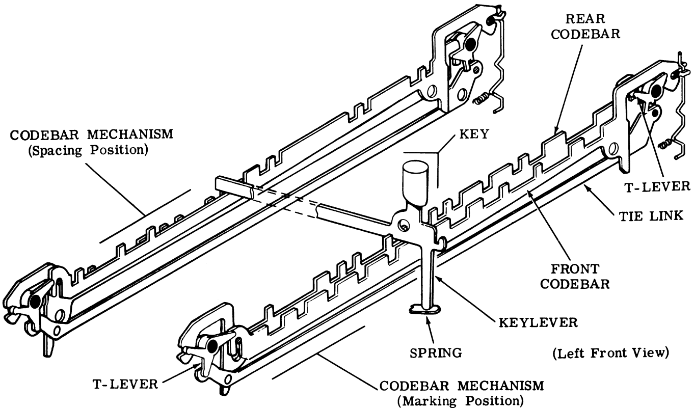
Figure 4 - Codebar Mechanism
