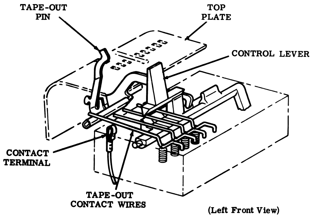
Figure 17 - Tape-Out mechanism
