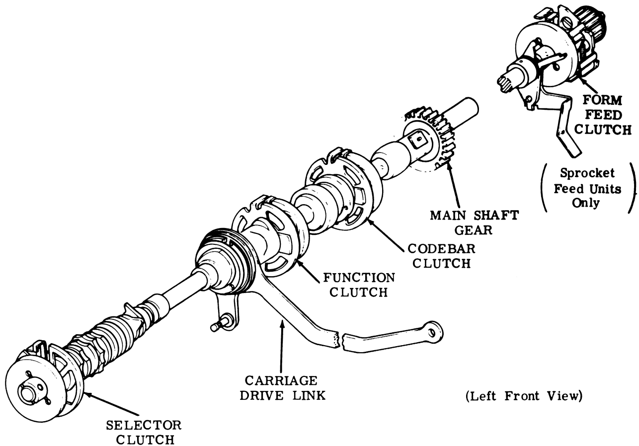
Figure 6 - Main Shaft
