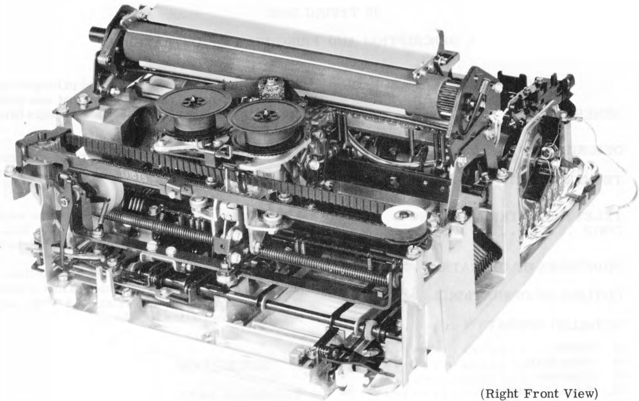
Figure 1 - 33 Typing Unit
