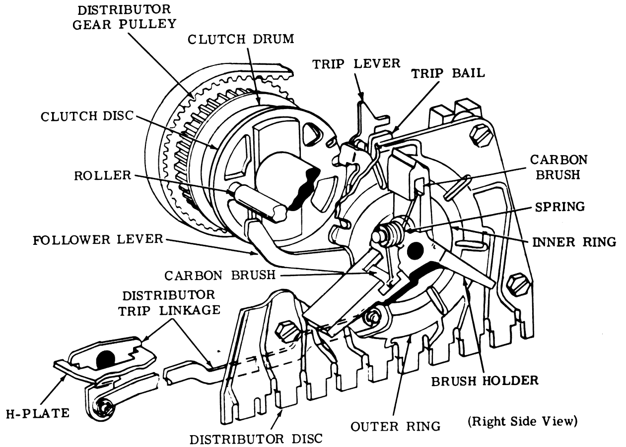
Figure 8 - Distributor Mechanism
