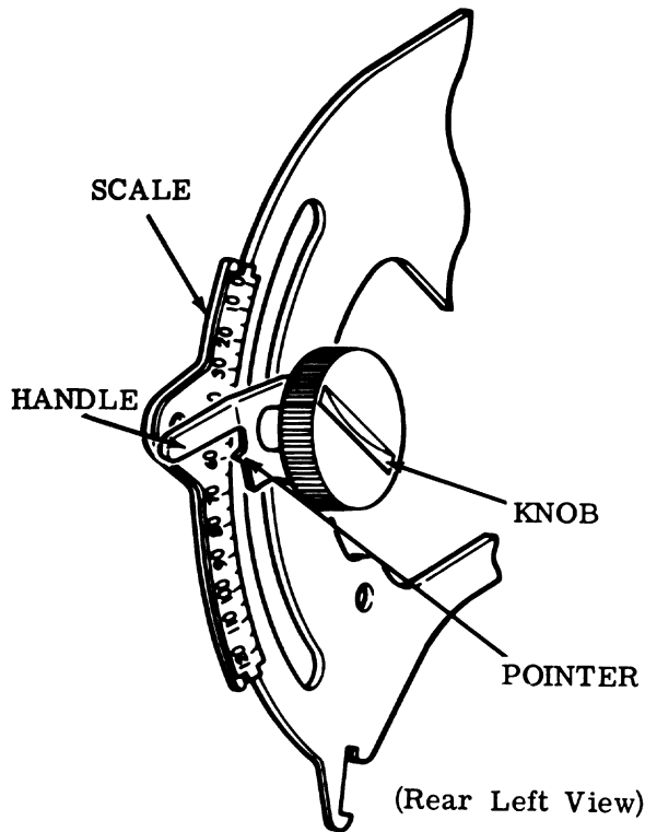
Figure 14 - Range Finder
