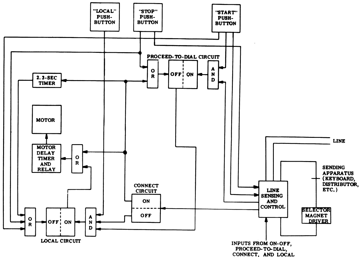
Figure 7 - Circuit Interconnections
