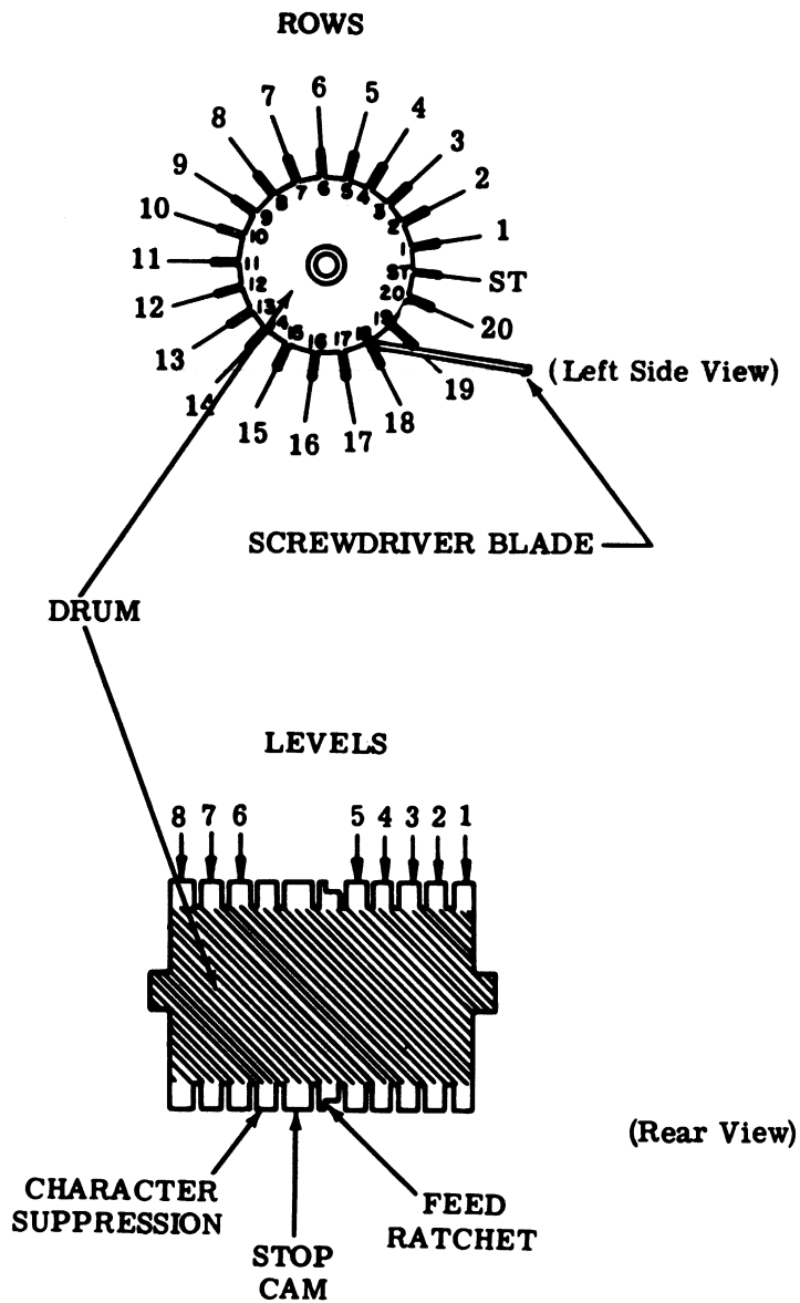
Figure 4 - Answer-Back Drum
