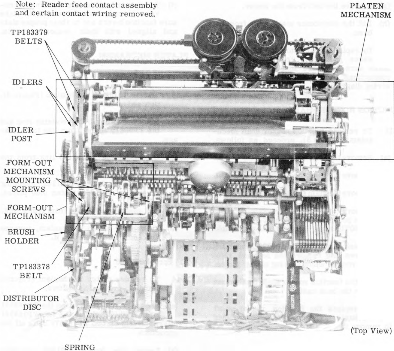
Figure 5 - Typing Unit
