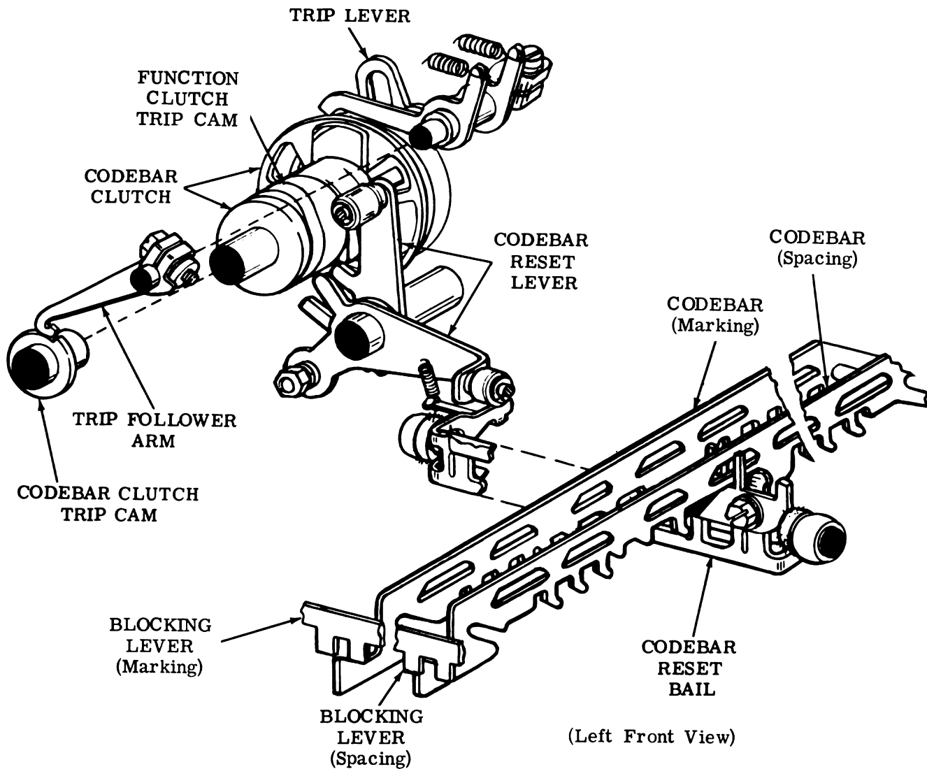
Figure 16 - Codebar Mechanism
