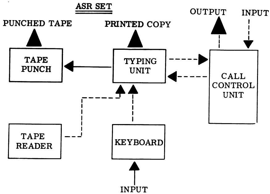
Figure 4 - Block Diagram of 33 Sets
