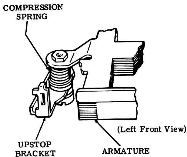
Figure 14 - Upstop Mechanism
