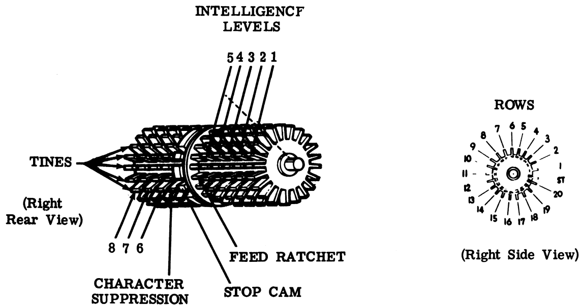
Figure 34 - Answer-Back Drum
