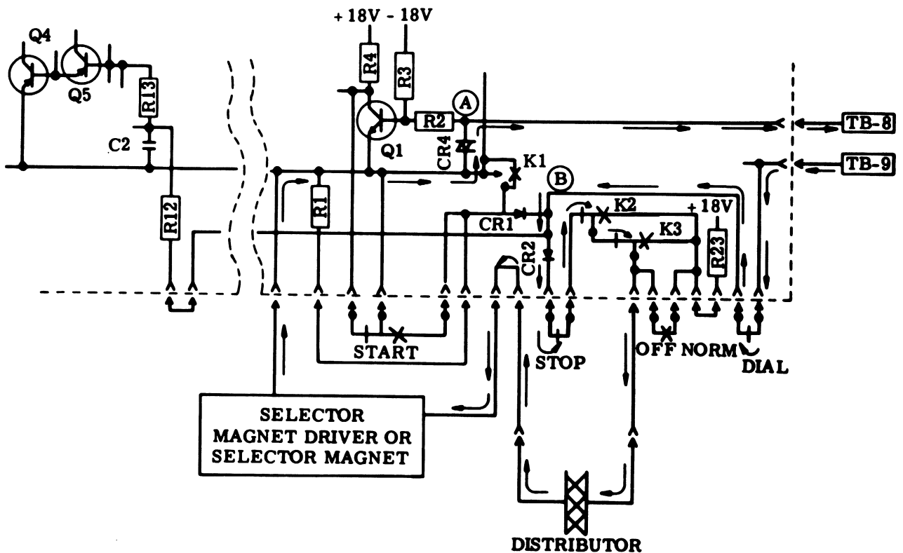
Figure 9 - Local-Remote Control Circuit – Current Flow (Local Connection)
