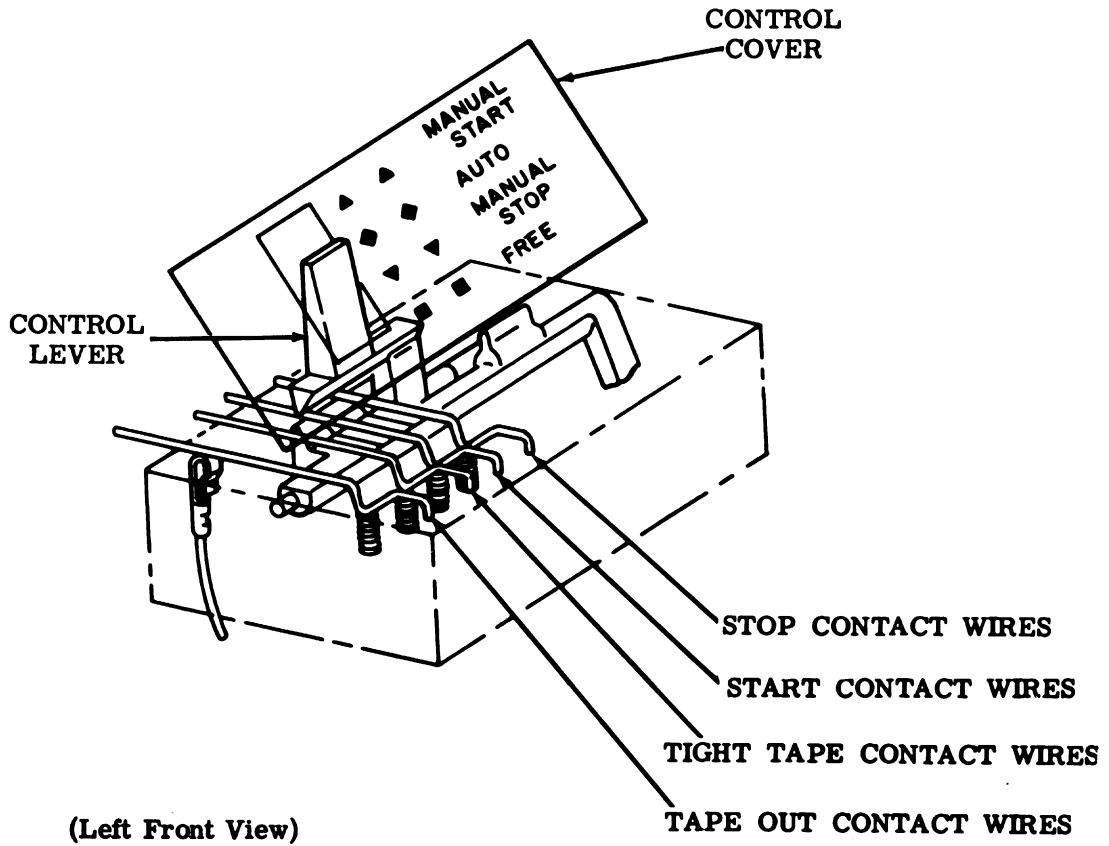
Figure 4 - Control Mechanism
