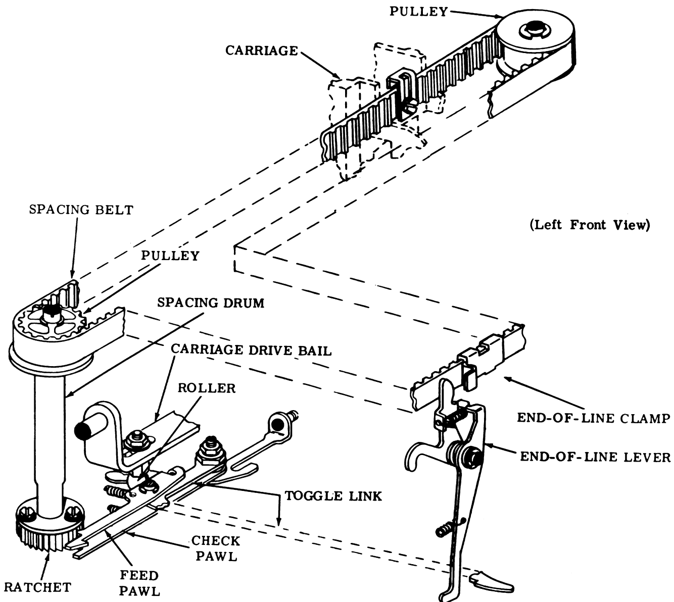
Figure 27 - Spacing Mechanism
