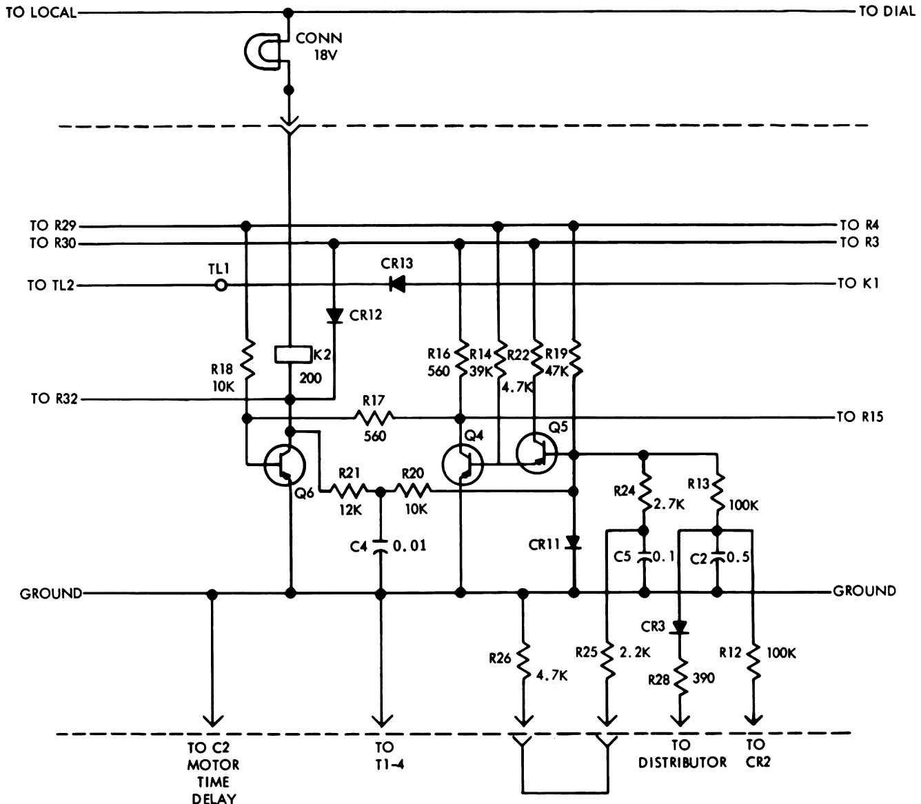
Figure 3 - Connect Circuit
