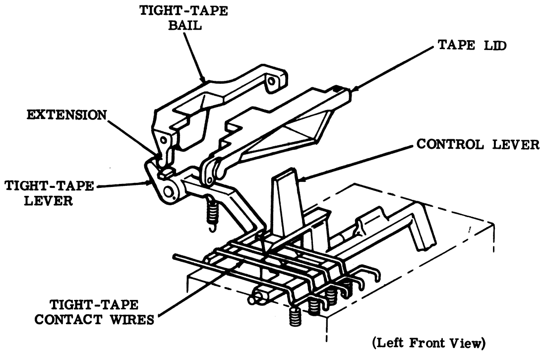
Figure 16 - Tight-Tape Mechanism
