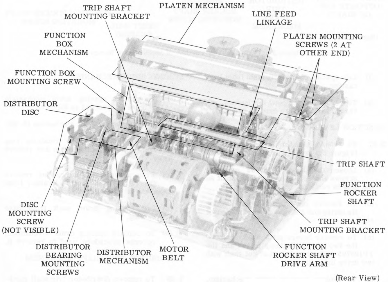
Figure 4 - Typing Unit
