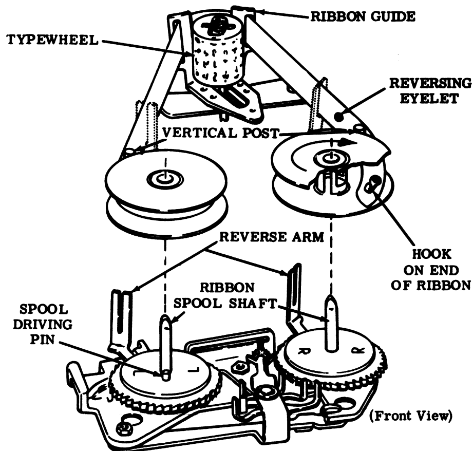
Figure 6 - Ribbon Threading
