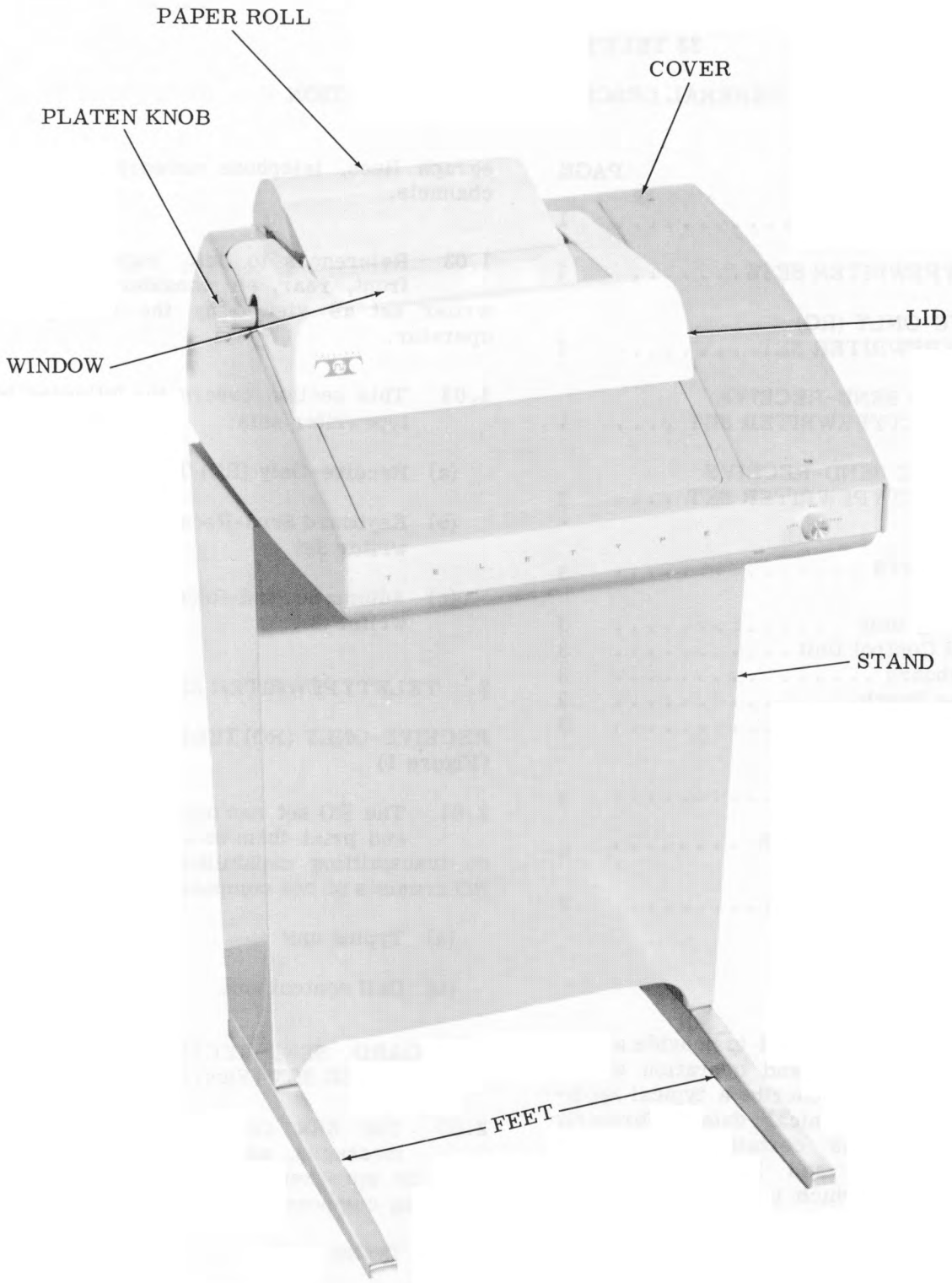
Figure 1 - Model 33 Receive-Only (RO) Teletypewriter Set
