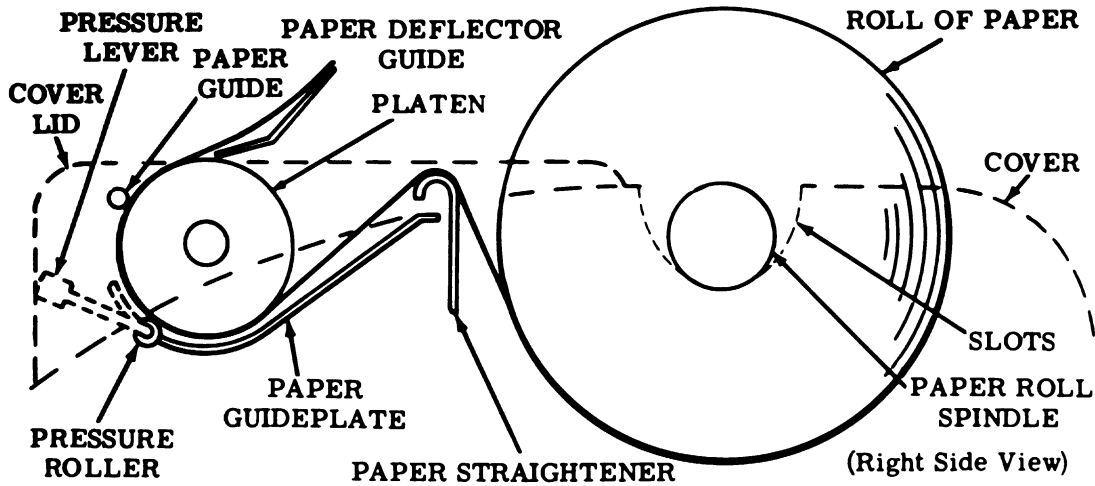
Figure 7 - Paper Threading — Friction Feed
