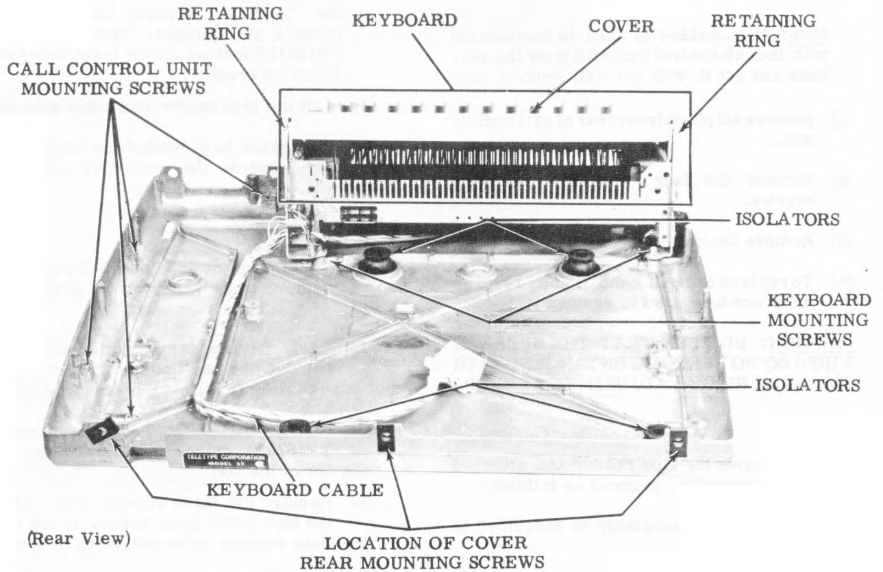
Figure 3 - Subbase With Keyboard
