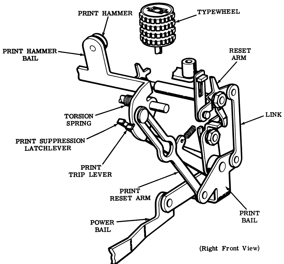
Figure 24 - Printing Mechanism
