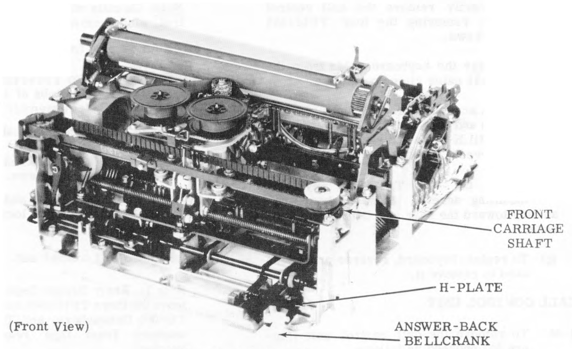
Figure 2 - Typing Unit
