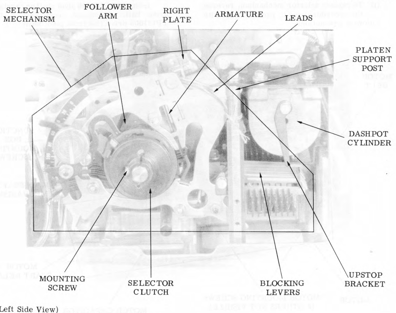
Figure 6 - Selector Mechanism
