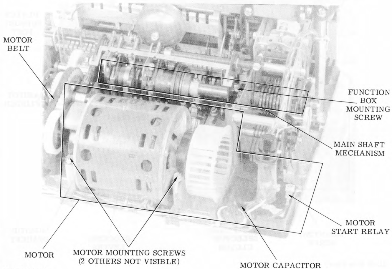
Figure 7 - Typing Unit
