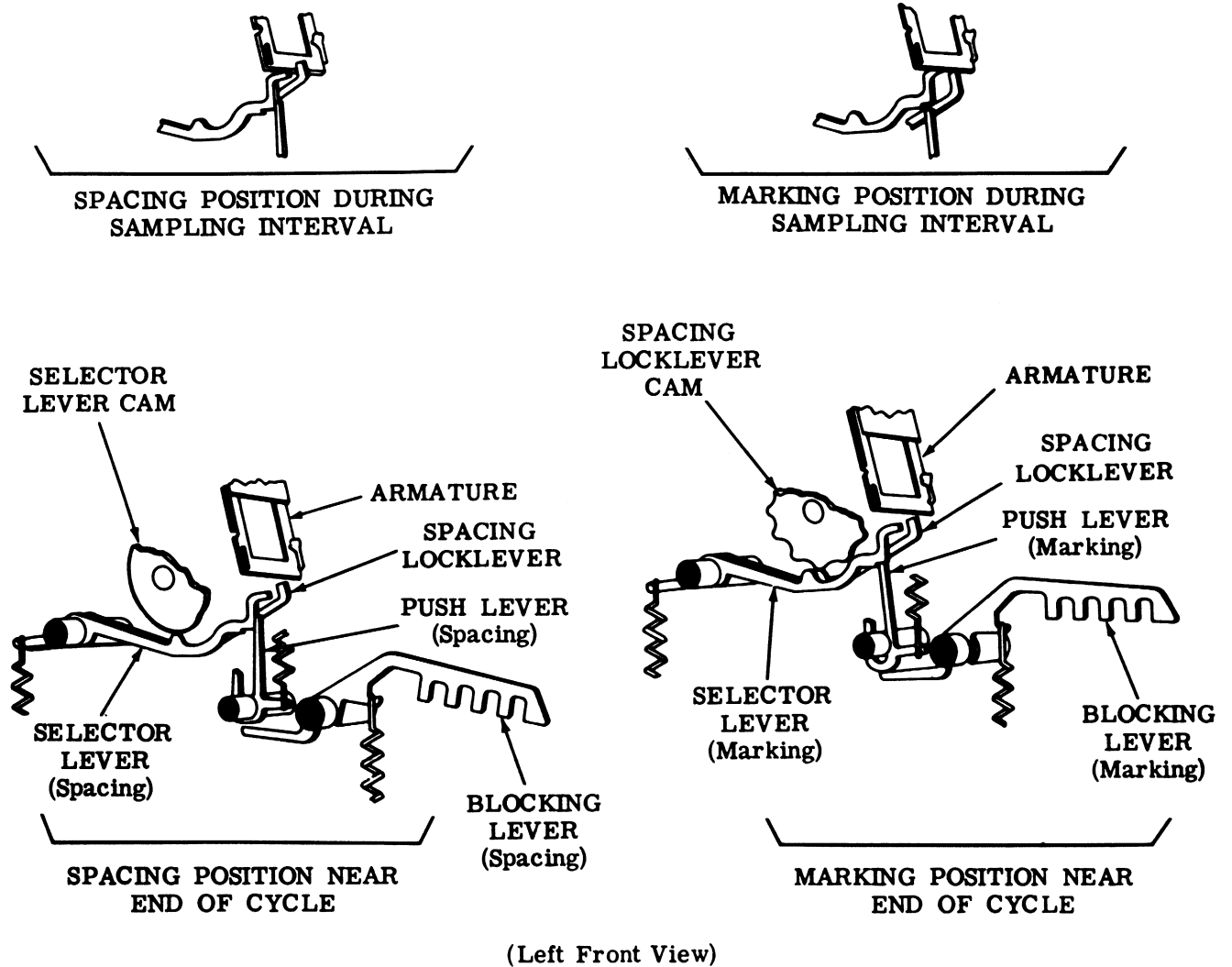
Figure 13 - Selector Mechanism
