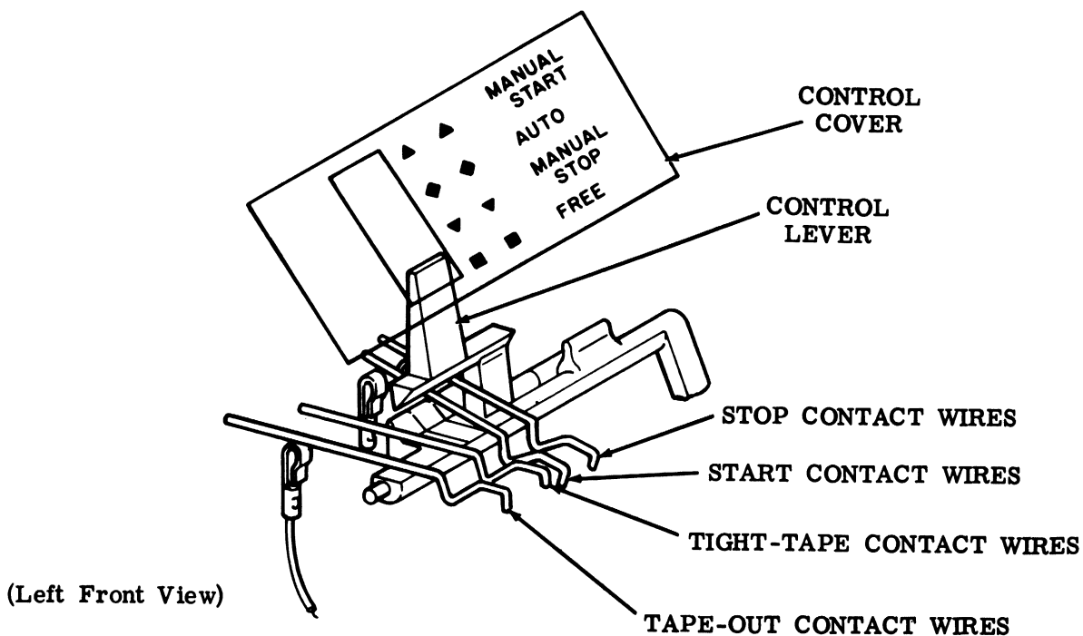
Figure 20 - Control Lever in FREE Position
