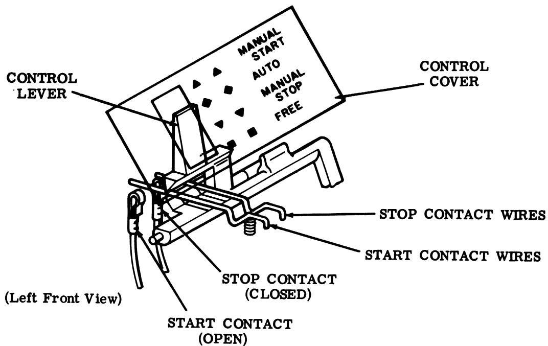
Figure 19 - Automatic Start Position
