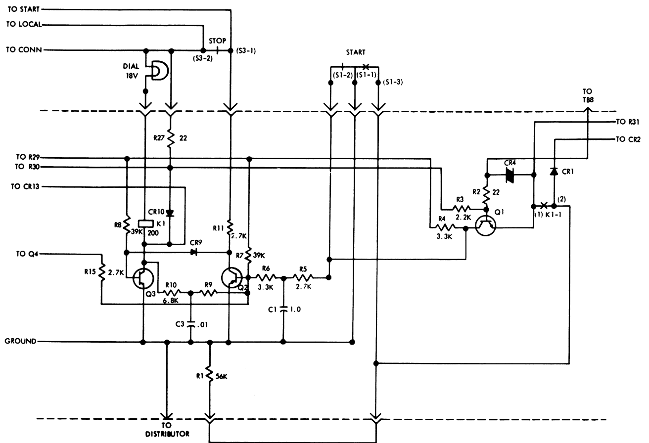
Figure 2 - Proceed-to-Dial Circuit
