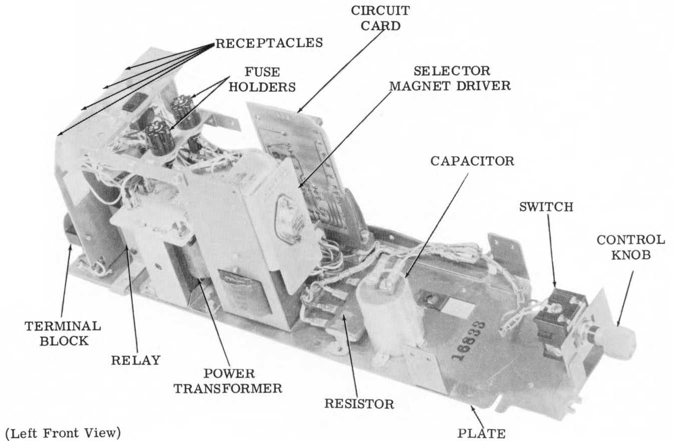
Figure 4 - Call Control Unit for Private Wire Service
