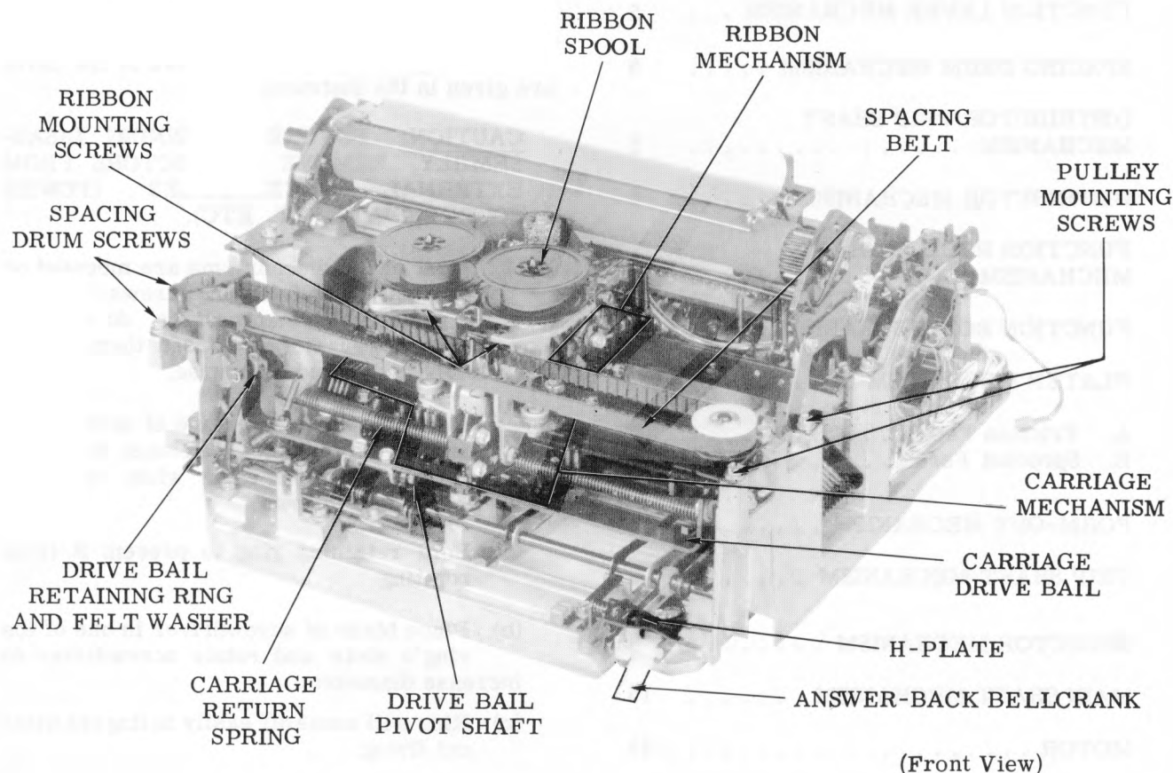
Figure 1 - Typing Unit
