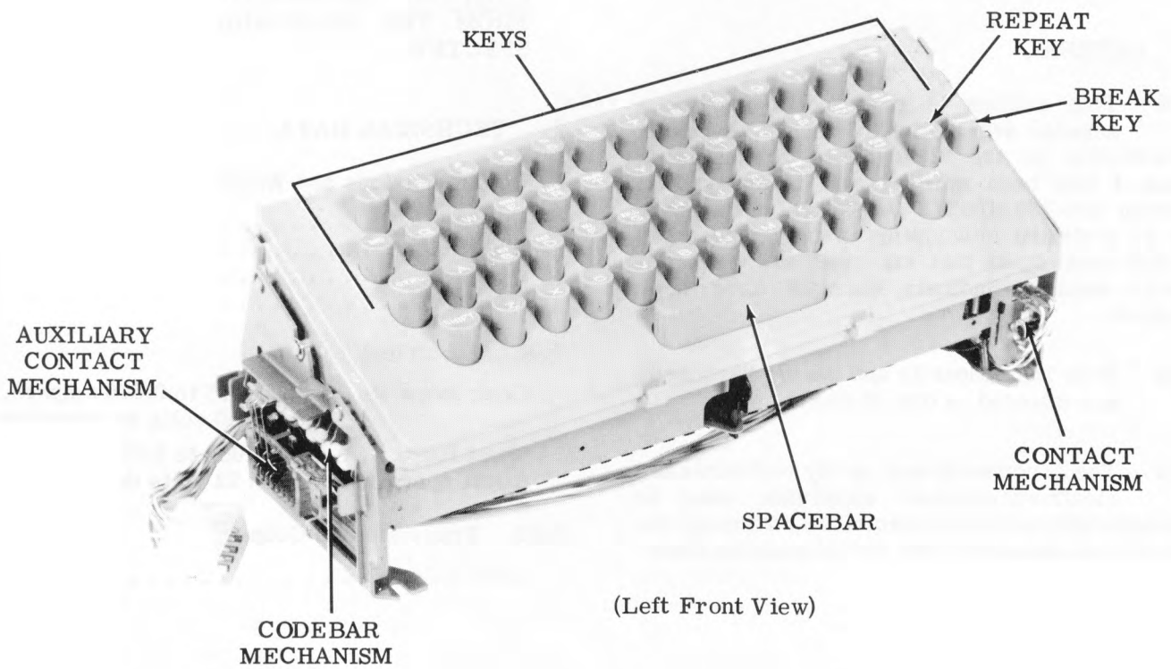
Figure 2 - Parity Keyboard
